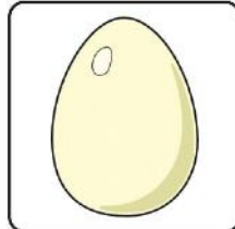
3. __gg
