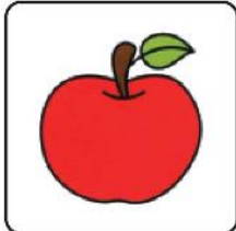
1. ___pple
